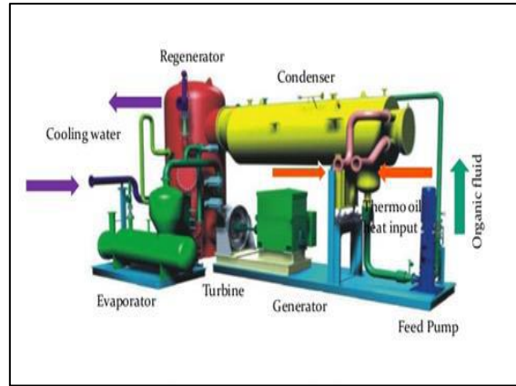
Fig. 3. ORC Components [2]
